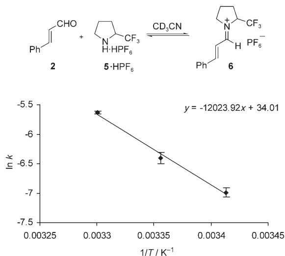
Figure 2. Arrhenius plot for iminium ion formation, with standard error of mean shown as error bars.
