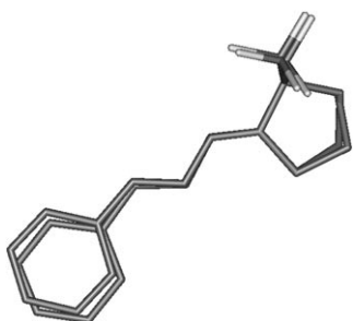
Figure 3. Overlay of X-ray and DFT structures of iminium ion 6 ; hydrogen atoms are omitted for clarity. Full crystal and geometrical details are reported in the Supporting Information.
