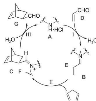
Figure 1. Proposed catalytic cycle for the iminium ion catalyzed Diels–Alder reaction. Labels A–C follow the species containing the catalytic amine group; labels D–G follow the species incorporating the starting \alpha,\beta -unsaturated carbonyl compound.
