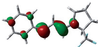
Figure 5. LUMO of iminium ion derived from 5 , with isosurface plotted at 0.05 au.
