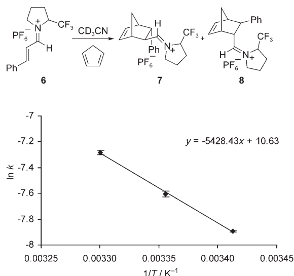
Figure 4. Arrhenius plot for the Diels–Alder cycloaddition, with standard error of mean shown as error bars.
